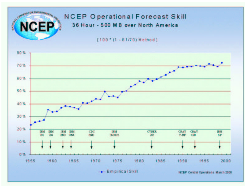
Figure 4. Skill of the 36 hour 500 hPa forecast produced at NCEP. Forecast skill is expressed as a percentage of an essentially perfect forecast score, for the period 1955–1999. The accuracy of prediction is closely linked to the available computer power; the introduction of new machines is indicated in the figure. Thanks to Bruce Webster of NCEP for the graphic of S_1 scores.
